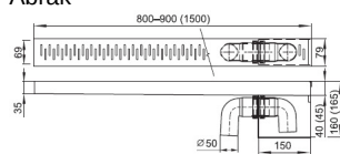
STANDARD DESIGNS OF GRATING
